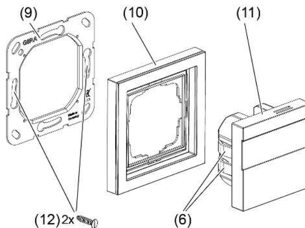
Figure 5: Mount device
